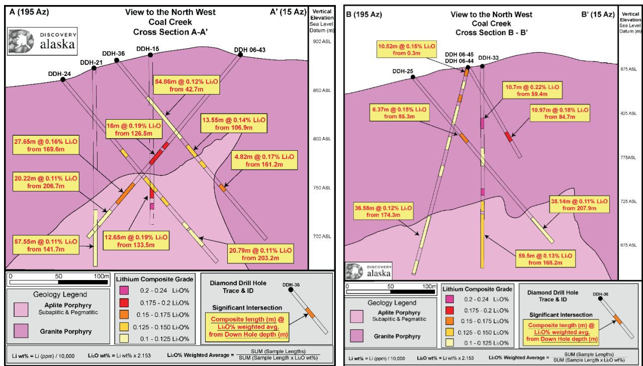
Figures 1-2. Coal Creek Cross Section A-A' & B-B' showing lithium intervals
